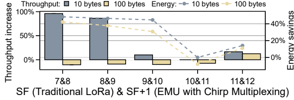
Figure 16: Performance when multiplexing chirps using EMU with a higher spreading factor (SF+1) than that used by traditional LoRa (SF) in a LoRaWAN context. When transmitting short payloads, EMU still achieves a higher throughput.
