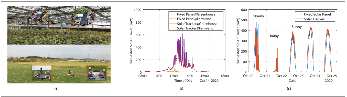
FIGURE 1. Case study of solar energy harvesting in agriculture. The TES-1333R data logging solar power meters were used to measure solar irradiance as a reference. The size of mini solar panels are 80 \times 55 mm. The converted current and voltage were measured using Adafruit INA219 breakout boards. Light tracers were used to demonstrate that the maximum energy can be harvested; a) two typical agricultural scenarios: greenhouse and farmland; b) corresponding results of harvested solar power; c) results at an open field in five days.
