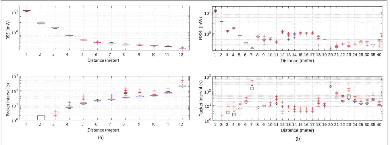
FIGURE 4. Evaluation of wireless power transfer using COTS Powercast system in line-of-sight scenarios: a) results in an open field; b) results in a hallway. RSSI is the abbreviation of received signal strength indicator.
