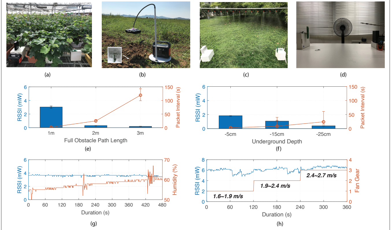
FIGURE 5. Evaluation of wireless power transfer using COTS Powercast system under different environmental conditions: a) plants are the obstacles between the TX91501B power transmitter and battery-free sensor node with a patch antenna; b) underground scenario, where the soil is the medium of wireless power transfer; c) irrigation affecting the microclimate; d) fan operation affecting the microclimate; e–h) the corresponding experimental results.
