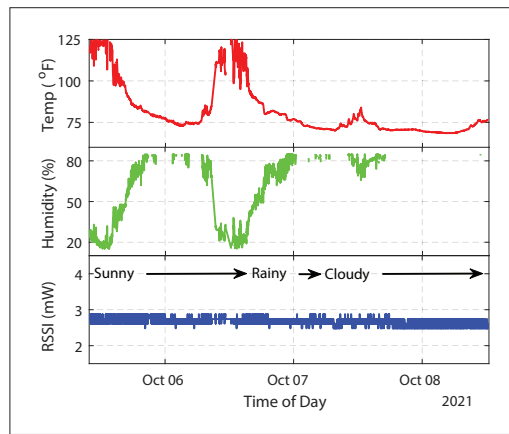
FIGURE 6. Evaluation of weather impact on wireless power transfer in a 74-hour outdoor deployment. The available measurement range of the used temperature sensor is between 25° F and 125° F, and the humidity sensor is between 15 percent and 85 percent.
